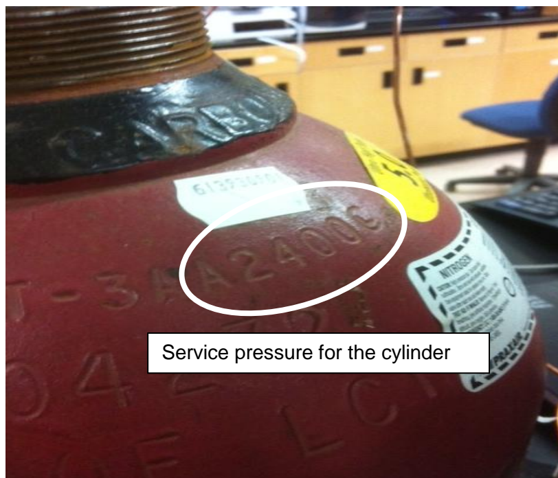
Figure 6: Service pressure for the compressed gas cylinder. Image courtesy of WSEP.
