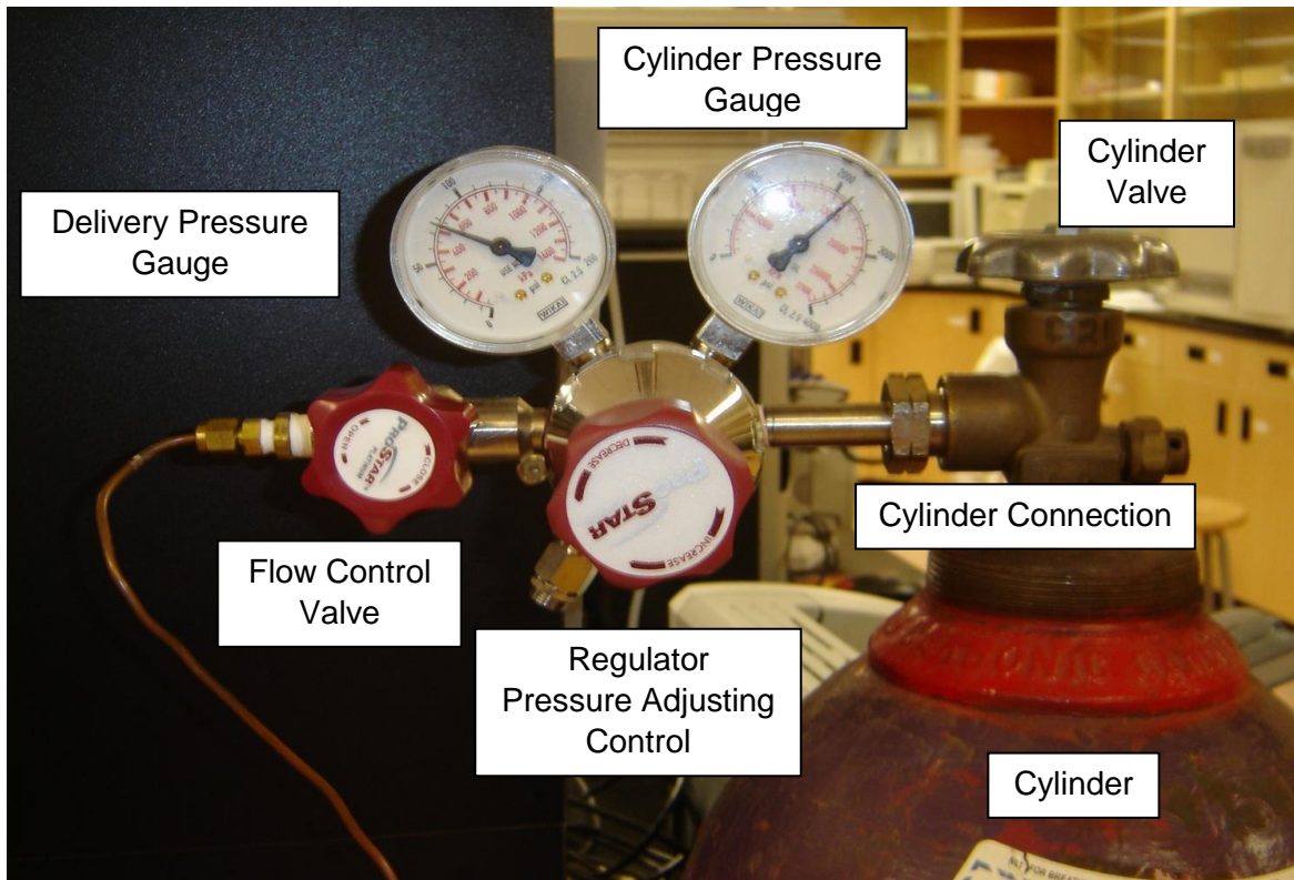
Figure 2. Main components of a compressed gas cylinder and regulator assembly. Image courtesy of WSEP.
